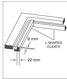
Support cleats
