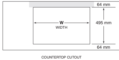
COUNTERTOP CUTOUT
