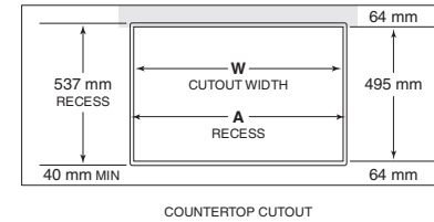
COUNTERTOP CUTOUT
