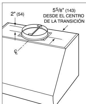
Descarga vertical
