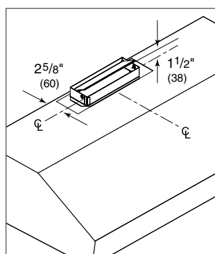
Vertical discharge
